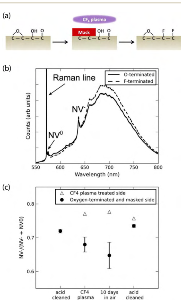
Fig. 5 Characterization of the impact of fluorine-terminated diamond on shallow NV centers. (a) Schematic showing use of CF 4 plasma to induce surface fluorination of oxygen-terminated diamond. (b) Representative photoluminescence spectra comparing oxygen- and fluorine-terminated surfaces. Zero-phonon lines (ZPL) of the NV 0 and NV − are indicated. (c) Ratio of the NV − ZPL area to that of the sum of NV − ZPL and NV 0 ZPL areas after different surface preparation conditions. Adapted with permission from ref. 259. Copyright 2013 AIP Publishing LLC.
